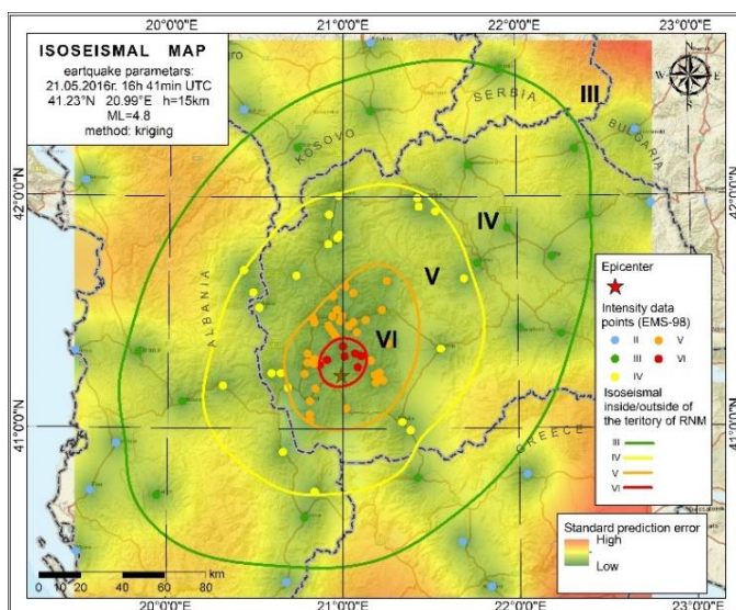
Figure 2. Iseismal map of the case study earthquake using kriging interpolation generated in ArcMap10.8.2
