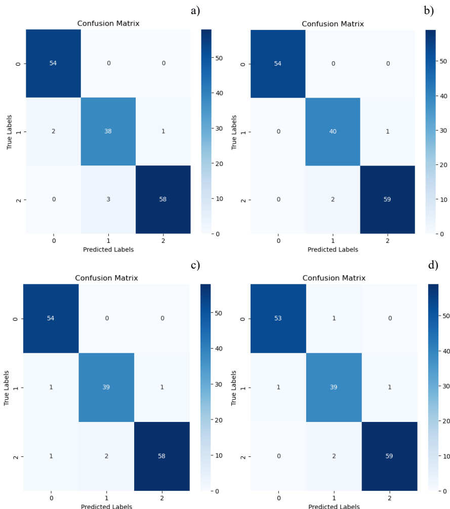
Figure 4: Confusion matrix for the first (a), second (b), third (c) and fourth (d) configuration
