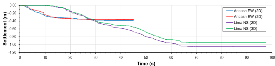
Figure 9. Time-history of settlement on the crest for the Ancash EW and Lima NS earthquakes
